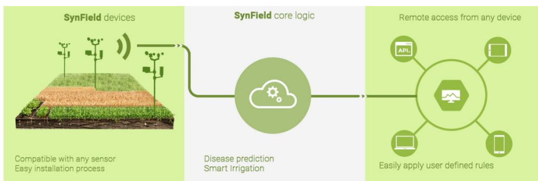
Figure 6: SynField ecosystem
